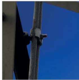
4 Downlead clamp
